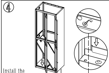
Install the bottom plate, then install the lower division plate in the same way
