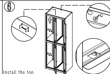
Install the top plate, then adjust the upper and lower division plate till fit well
