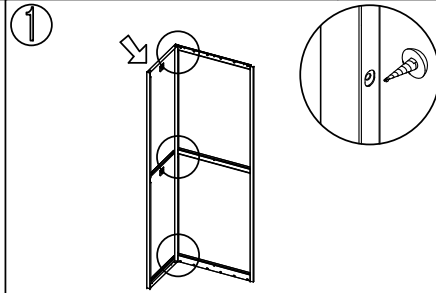
Bolt the left side and back plate with self-tapping screws(5x12)
