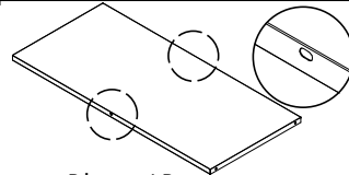
Bottom Plate:1Pc
