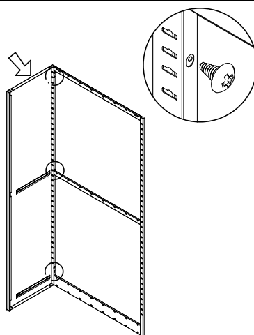
Bolt the left side and back plate with self-tapping screws(5x12)
