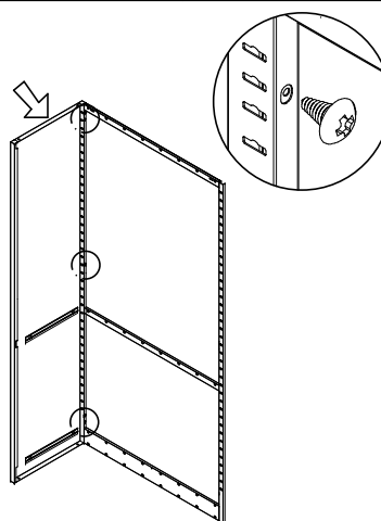
Bolt the left side and back plate with self-tapping screws(5x12)
