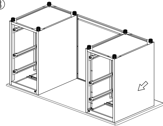
6*10 Screw: 6Pcs
