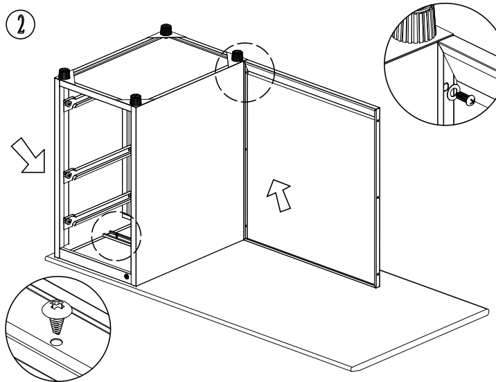
Back Plate: 1Pc
